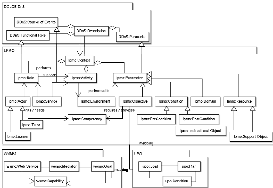
Figure 3. Conceptual model of parts of the LPMO and key mappings to the UPO and the WSMO framework.
