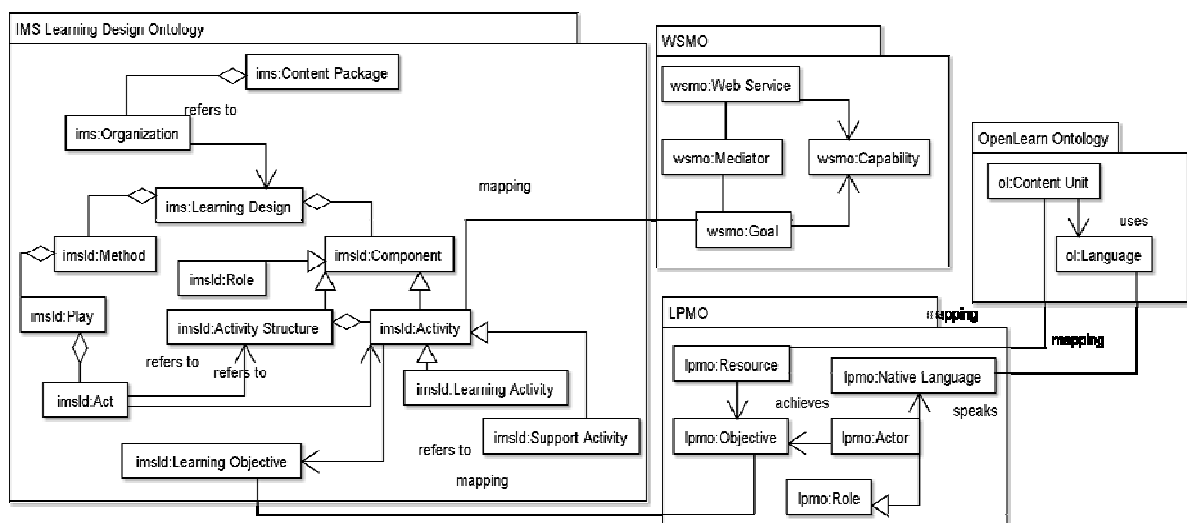
Figure 5. Ontological mappings implemented and utilized in the prototype application.
