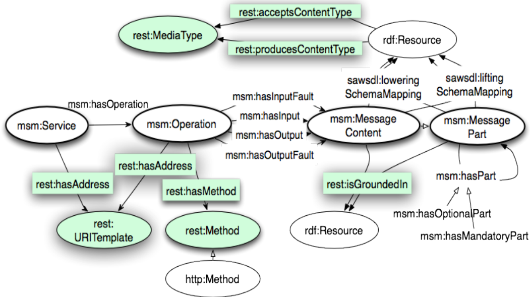
Fig. 1: Web API Grounding Model
